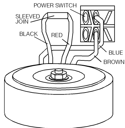
230V OPERATION
