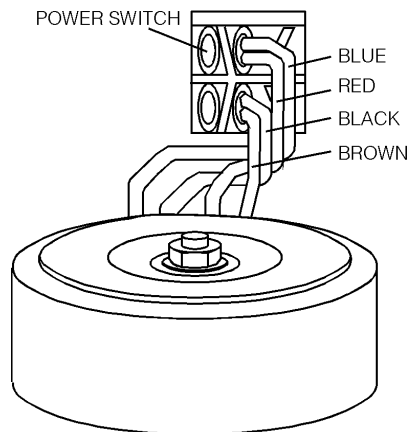
115V OPERATION
